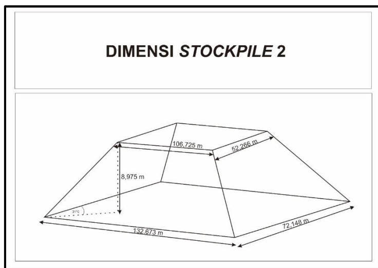
Gambar 3. Dimensi Stockpile 2
